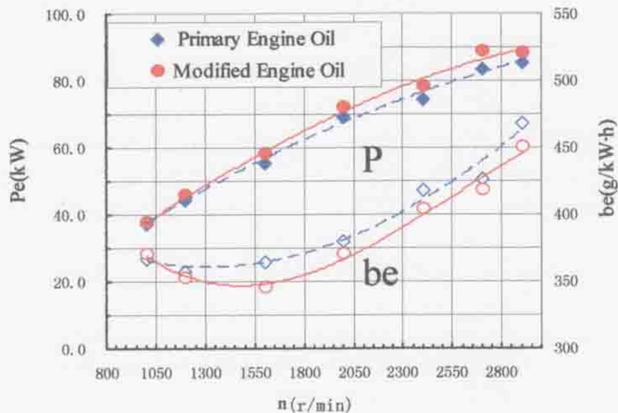
Fig. 1 Compare Curvere of Engine Output Property
