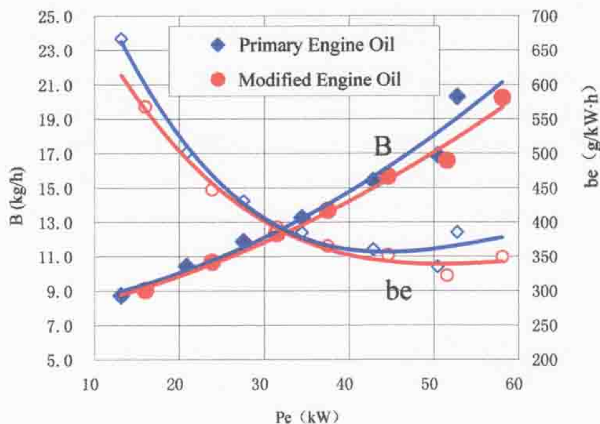
Fig. 2 Loading Property at 1600r/min
