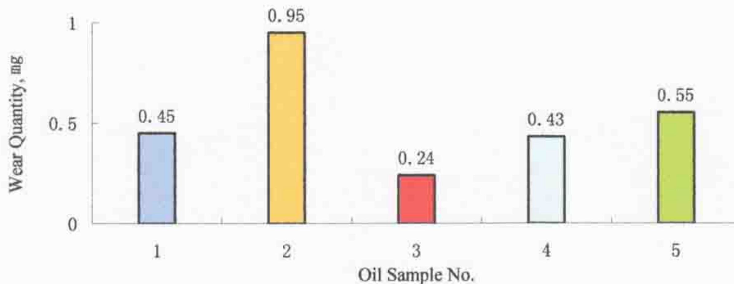
Fig. 3 The Wear Quantity of The Steel/Steel Friction-pair Loading with 240N
