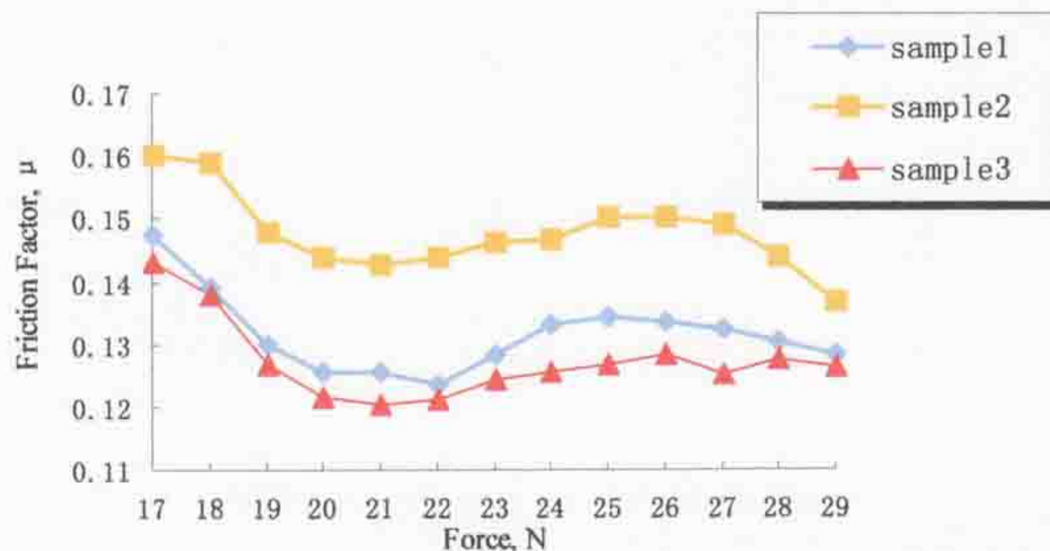
Fig. 4 The Varies of The Friction Factor with the Force for The Steel/Copper Friction-pair
